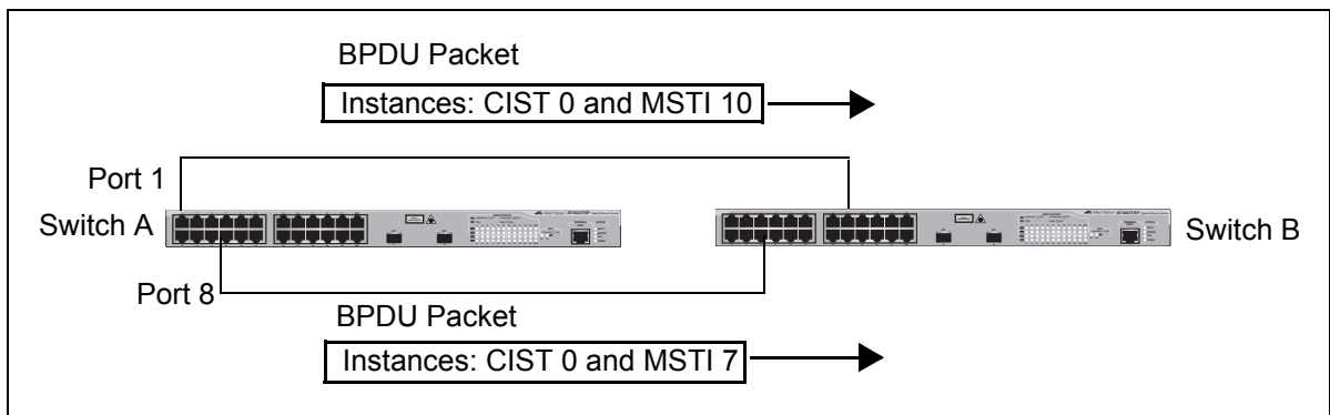
Figure 30. CIST and VLAN Guideline - Example 1
