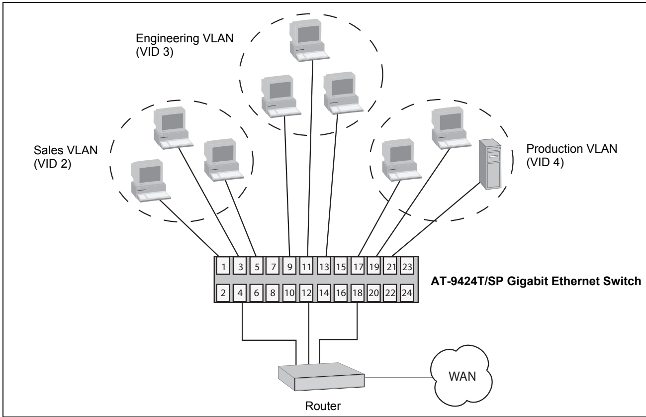
Figure 33. Port-based VLAN - Example 1
