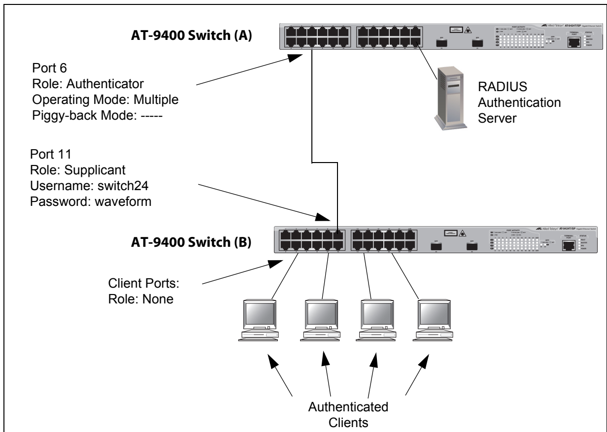
Figure 46. Authenticator Port in Multiple Operating Mode - Example 2
