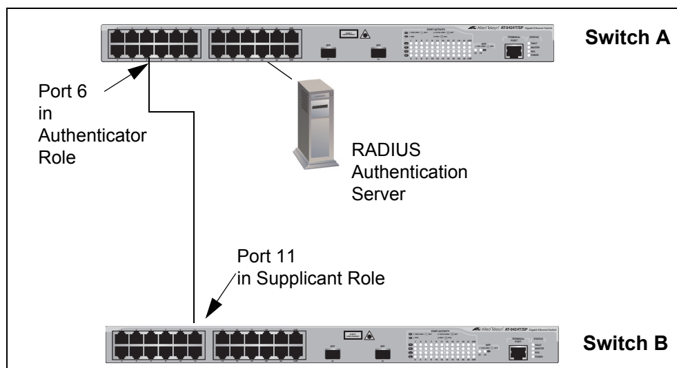
Figure 40. Example of the Supplicant Role
