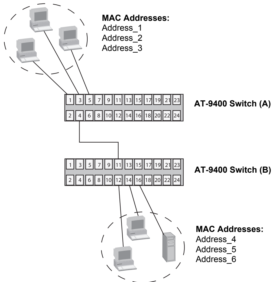
Figure 39. Example of a MAC Address-based VLAN Spanning Switches
