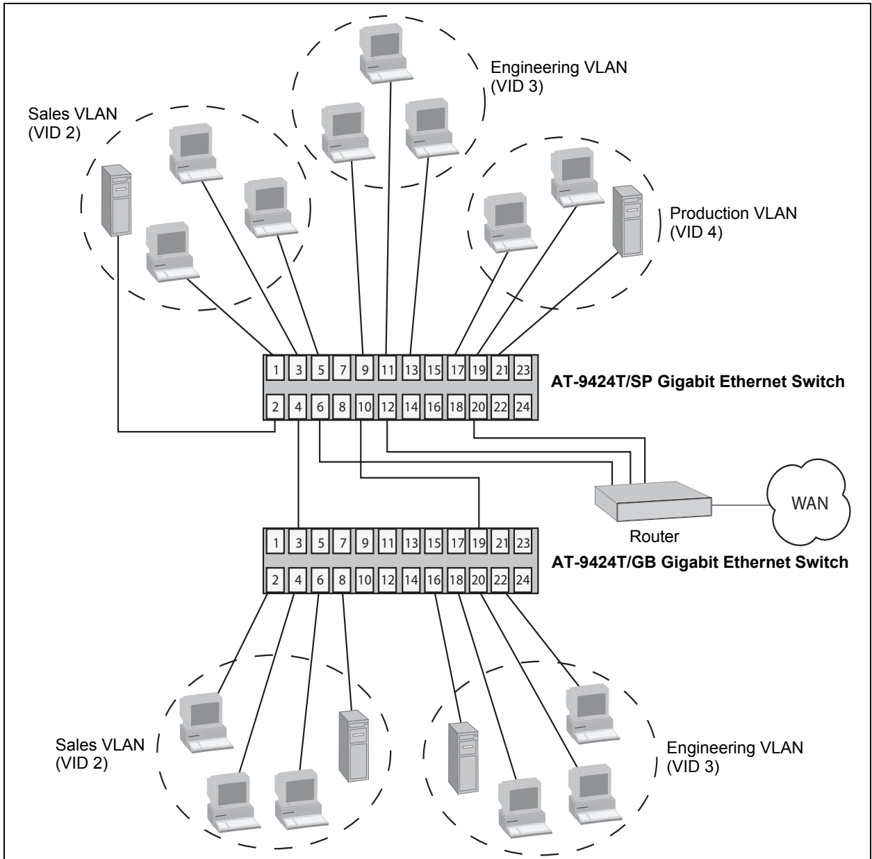
Figure 34. Port-based VLAN - Example 2
