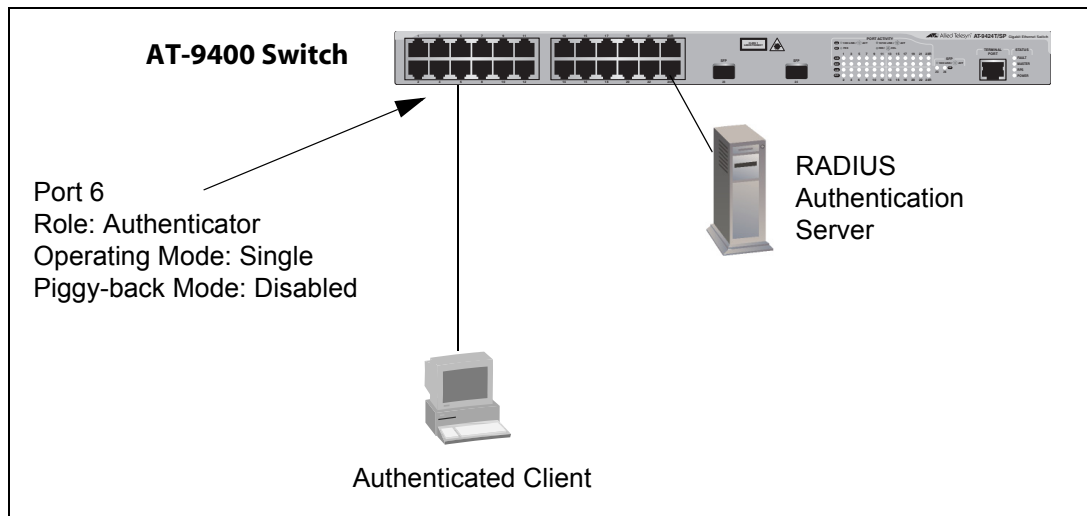
Figure 41. Authenticator Port in Single Operating Mode with a Single Client
