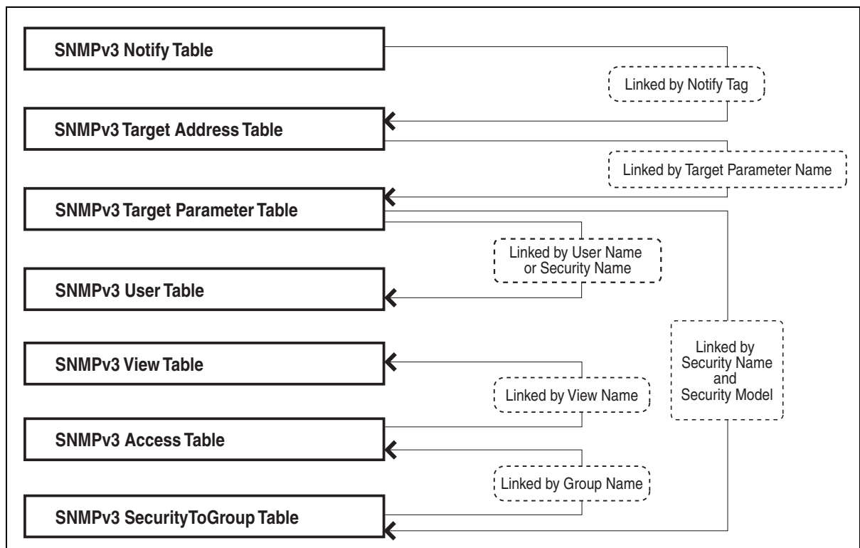
Figure 21. SNMPv3 Message Notification Process
