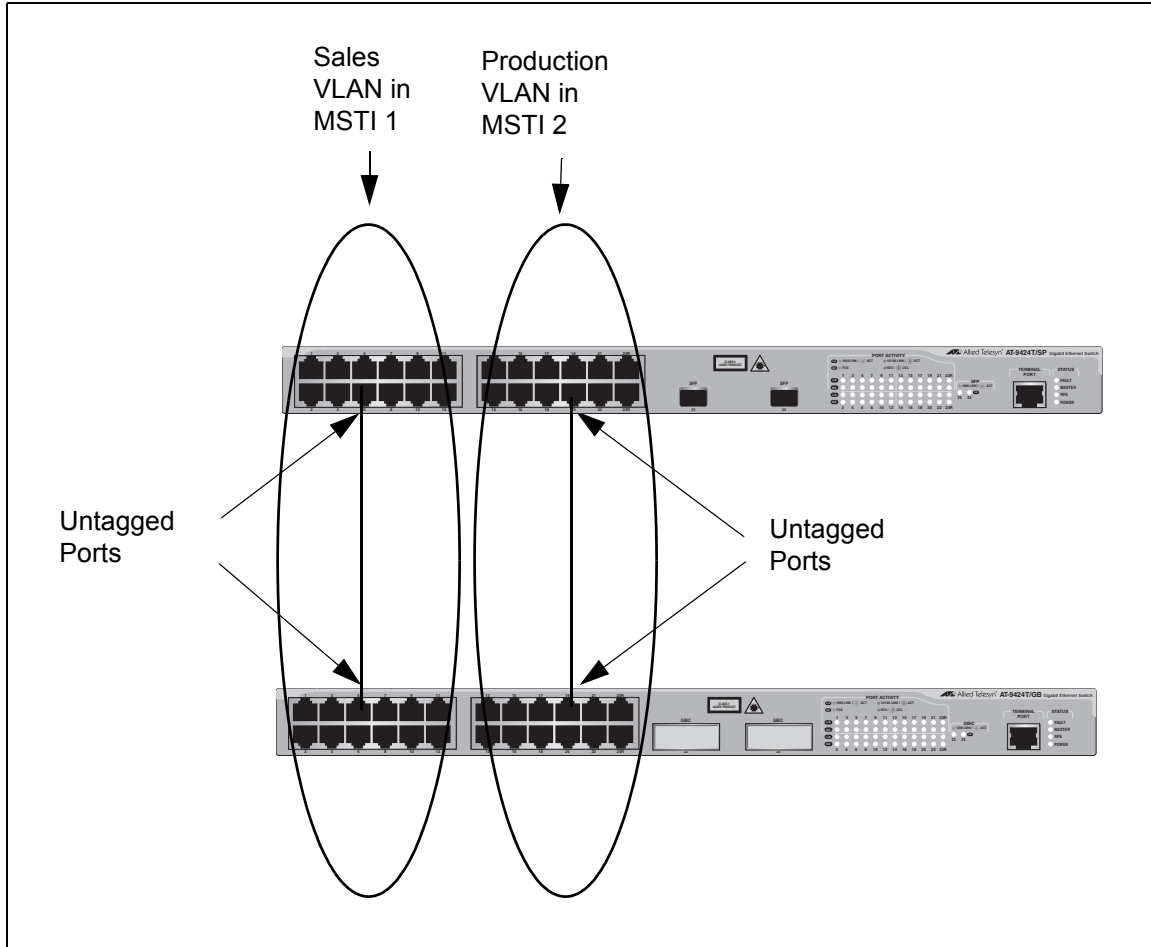
Figure 27. MSTP Example of Two Spanning Tree Instances
