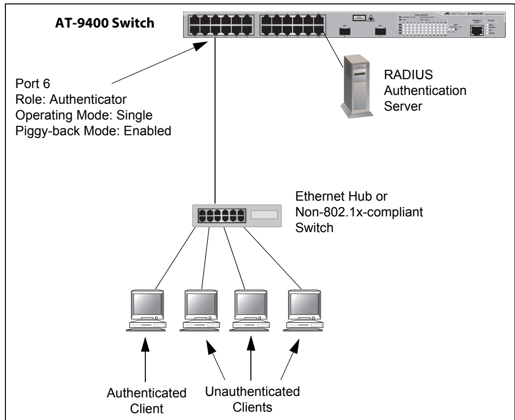
Figure 42. Single Operating Mode with Multiple Clients Using the Piggy-back Feature - Example 1
