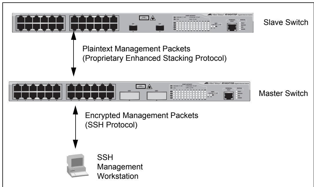
Figure 47 SSH Remote Management of a Slave Switch
