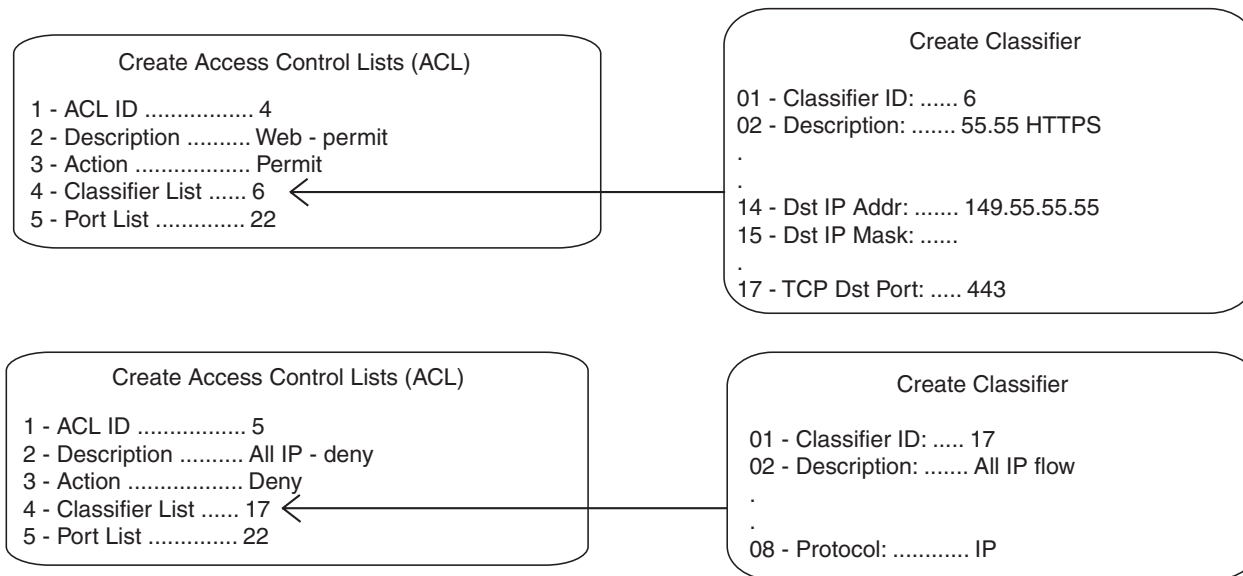
Figure 11. ACL Example 5
