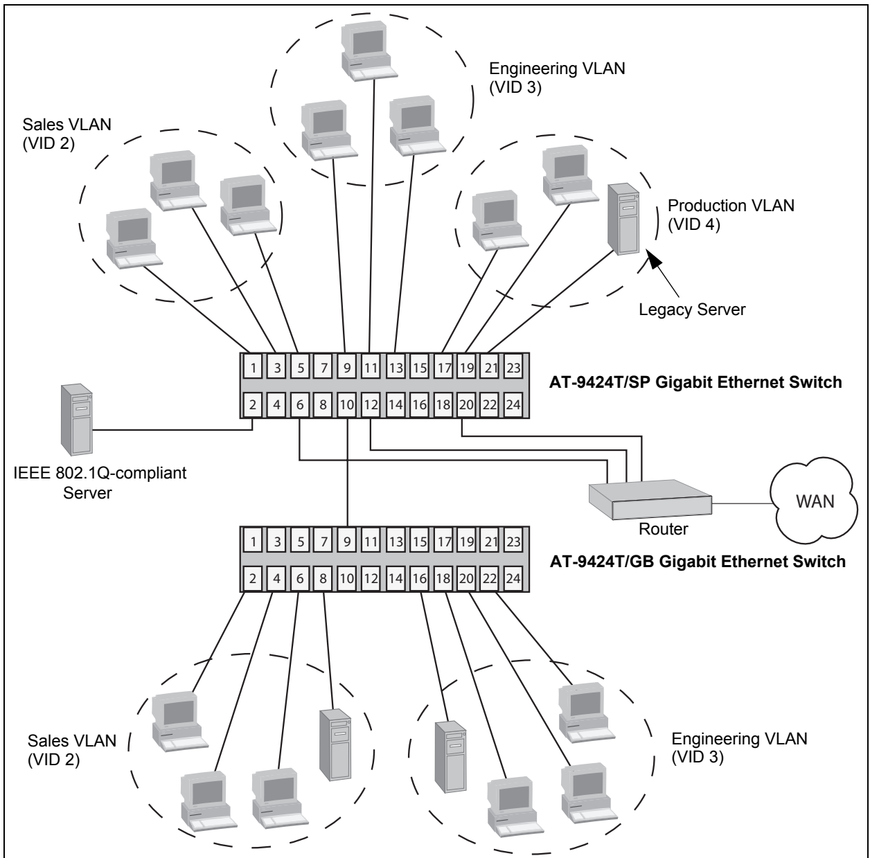
Figure 35. Example of a Tagged VLAN
