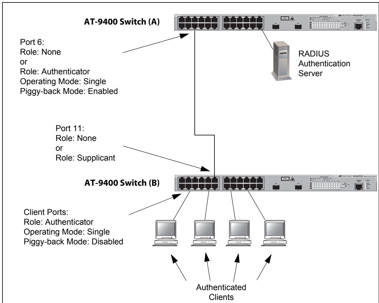
Figure 44. Single Operating Mode with Multiple Clients Using the Piggy-back Feature - Example 3
