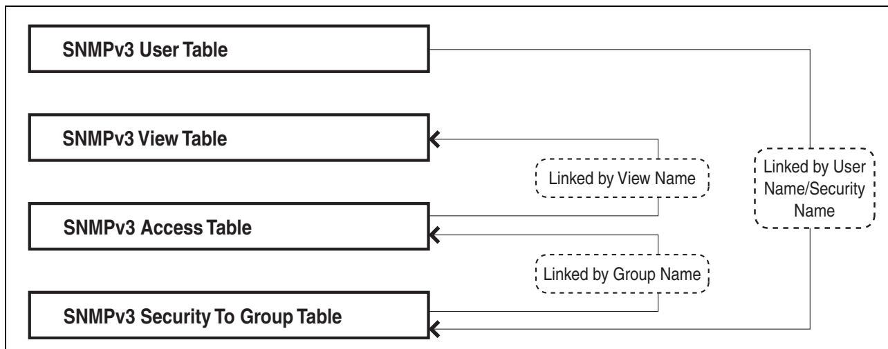
Figure 20. SNMPv3 User Configuration Process
