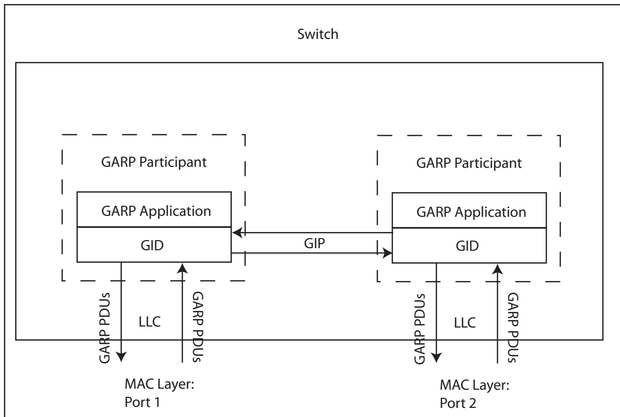
Figure 37. GARP Architecture
