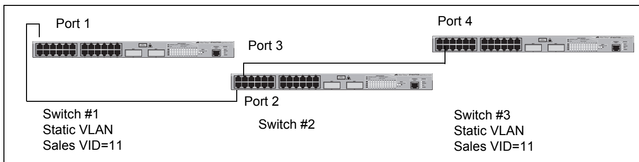
Figure 36. GVRP Example
