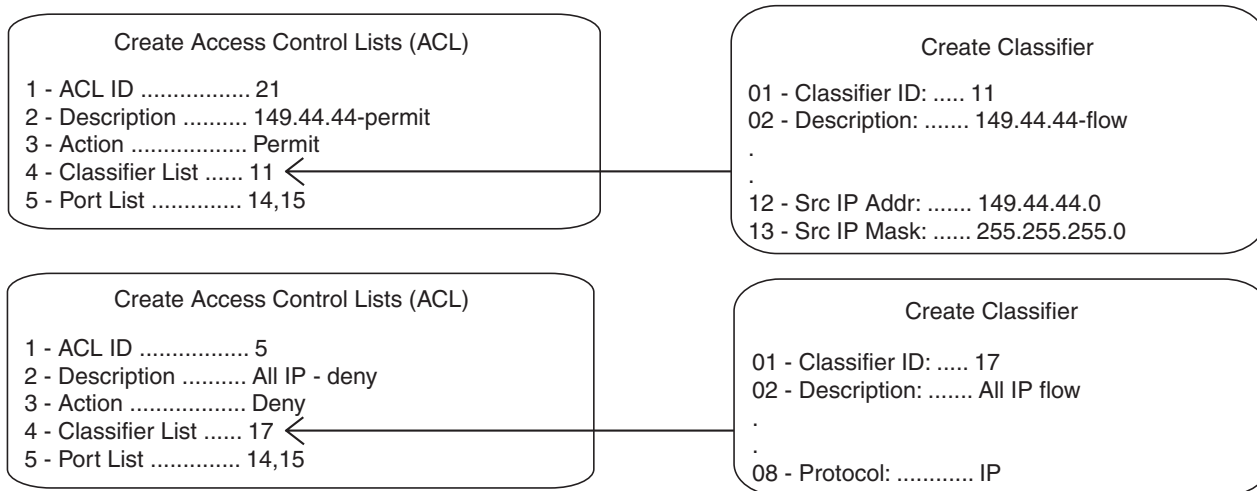
Figure 10. ACL Example 4
