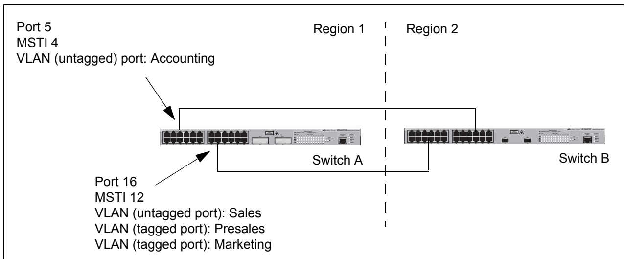
Figure 32. Spanning Regions - Example 1
