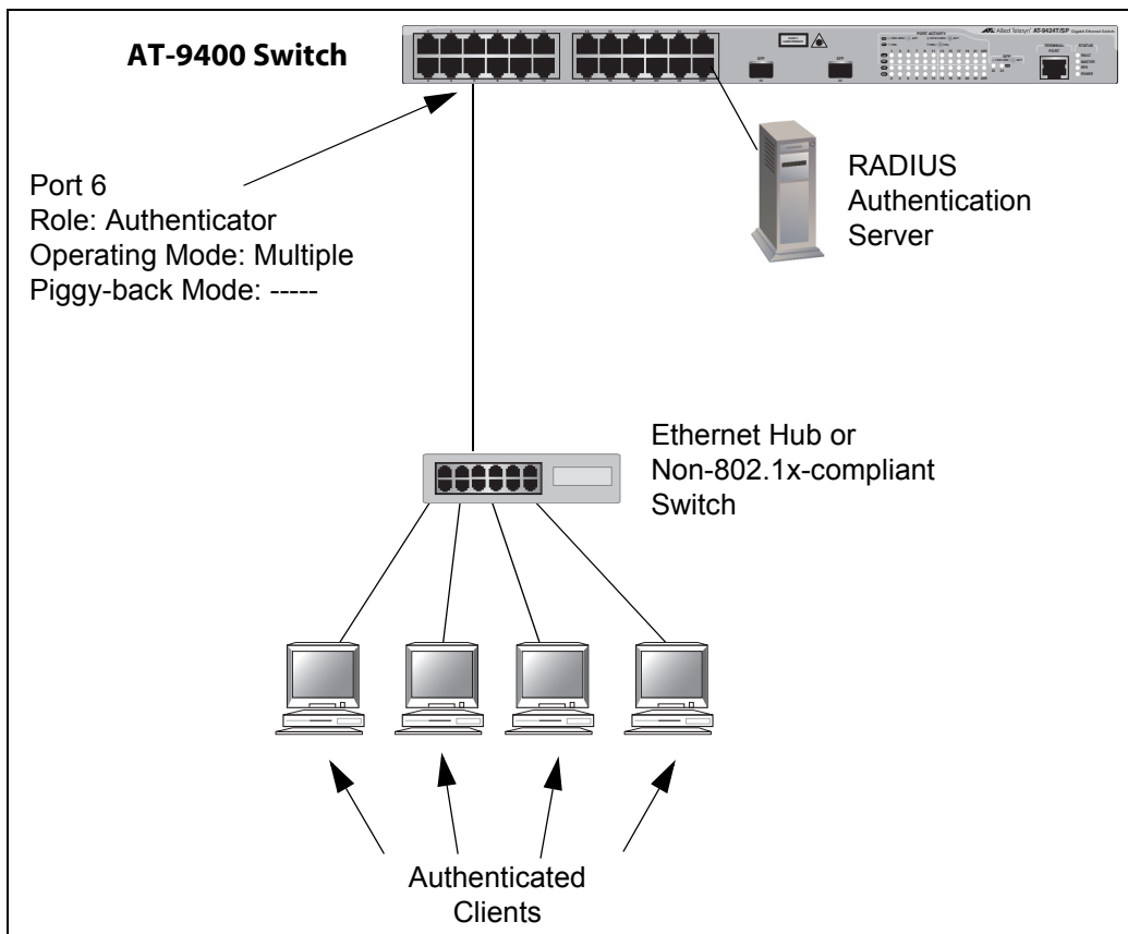
Figure 45. Authenticator Port in Multiple Operating Mode - Example 1
