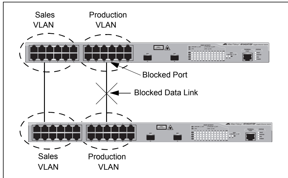
Figure 25. VLAN Fragmentation
