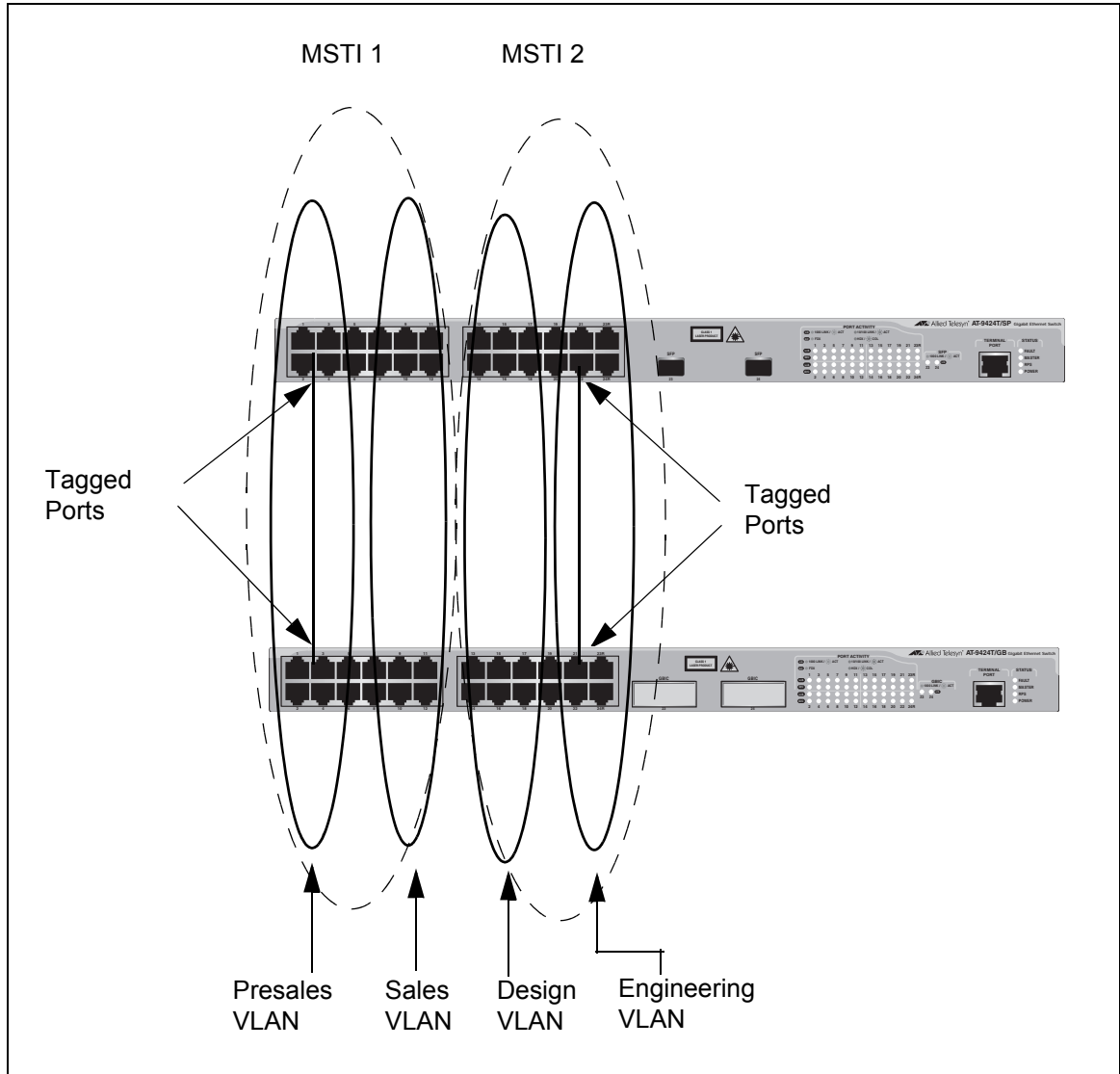
Figure 28. Multiple VLANs in a MSTI
