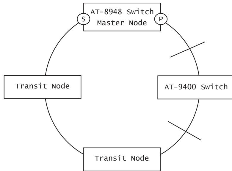
Figure 18. Double Fault Condition in EPSR Snooping
