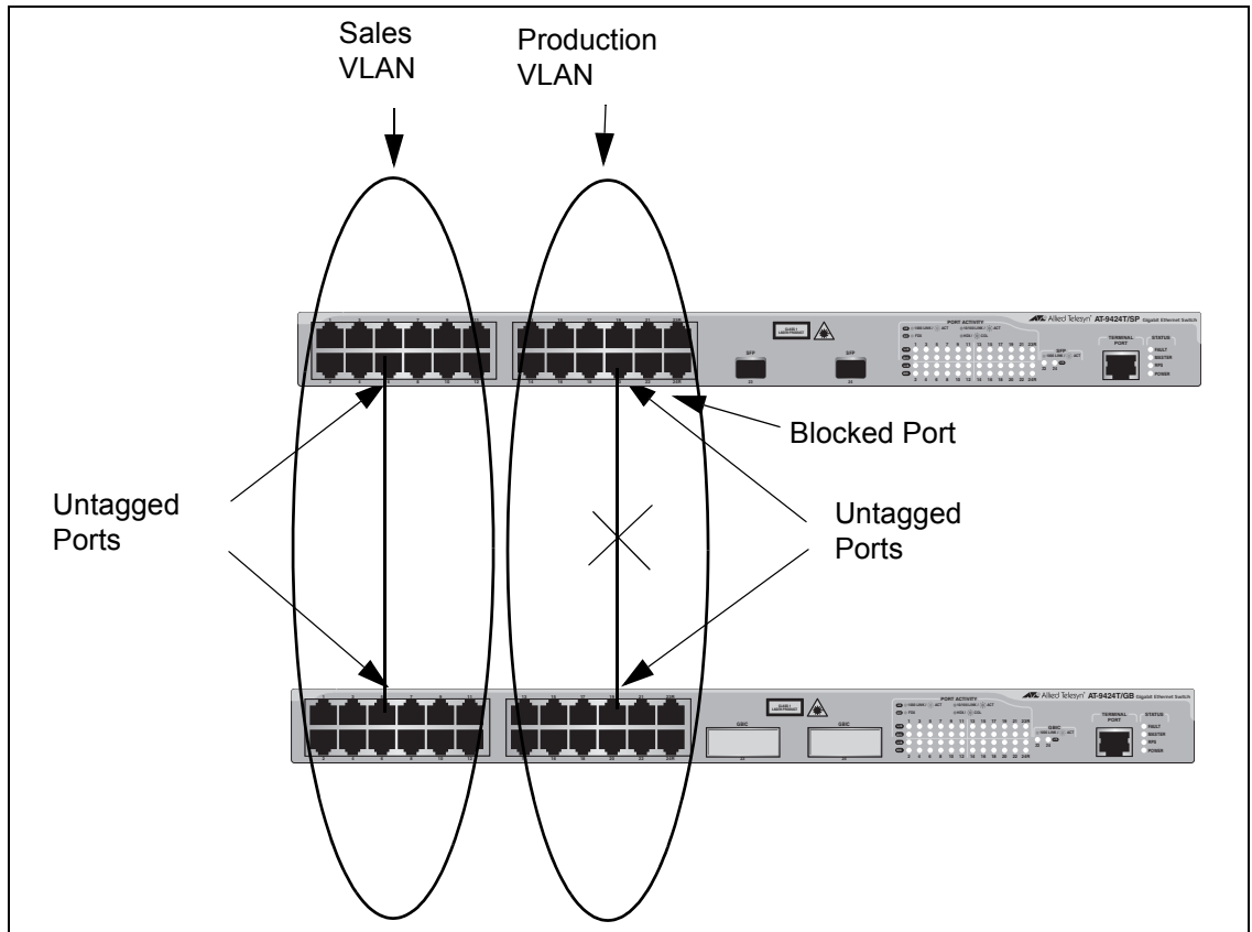
Figure 26. VLAN Fragmentation with STP or RSTP
