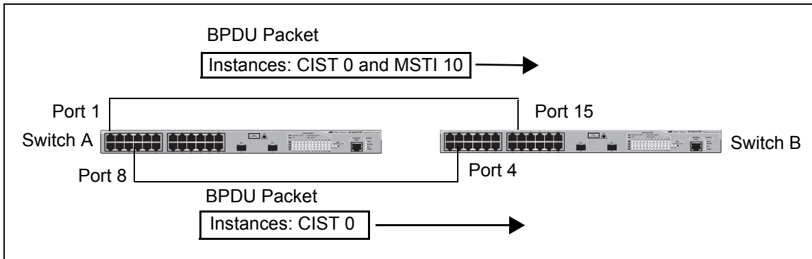
Figure 31. CIST and VLAN Guideline - Example 2
