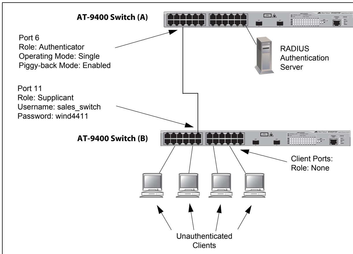
Figure 43. Single Operating Mode with Multiple Clients Using the Piggy-back Feature - Example 2
